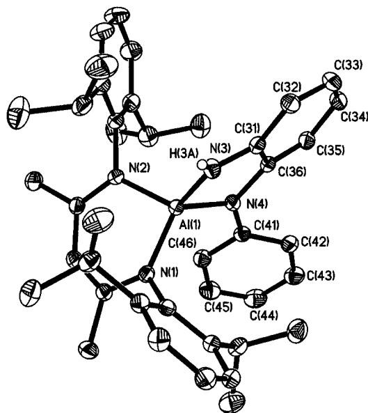
Figure 1. Molecular structure of compound 3 . The hydrogen atoms of the C–H bonds have been omitted for clarity. Selected bond lengths [ \text{\AA} ] and angles [ ^\circ ]: Al(1)–N(1) 1.862(1) , Al(1)–N(2) 1.893(1) , Al(1)–N(3) 1.807(2) , Al(1)–N(4) 1.847(1) , N(3)–C(31) 1.386(2) , C(31)–C(36) 1.429(2) , C(36)–N(4) 1.420(2) ; N(1)–Al(1)–N(2) 97.68(6) , N(3)–Al(1)–N(4) 90.39(6) , Al(1)–N(3)–C(31) 109.86(10) , N(3)–C(31)–C(36) 115.57(14) , C(31)–C(36)–N(4) 113.40(10) , C(36)–N(4)–Al(1) 108.44(10) .
