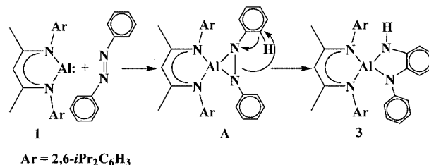
Scheme 1. Proposed formation of 3 from the reaction of 1 and \text{PhNNPh} .
